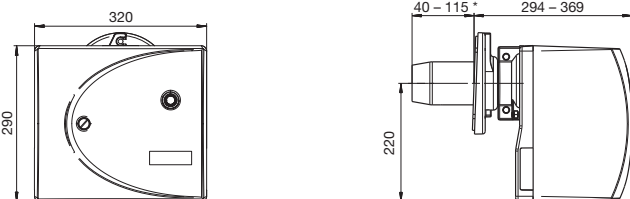
Sliding flange
